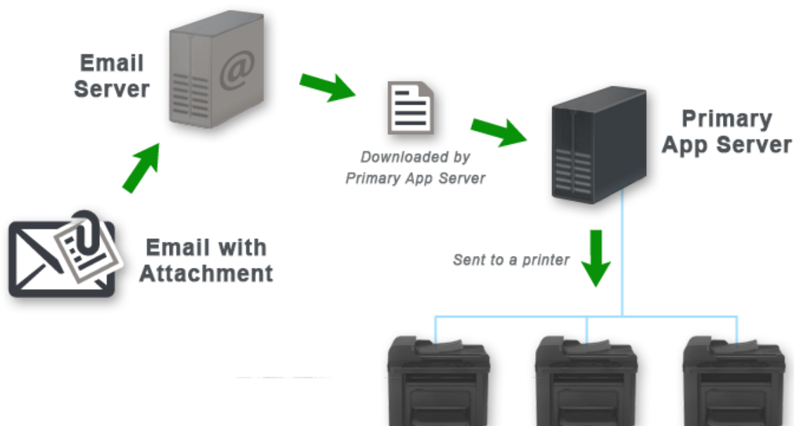
Figure 52: workflow
