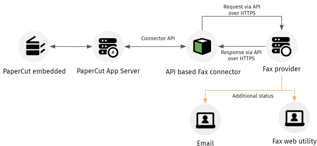
Scan to fax journey via API
