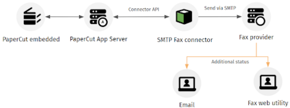
The Basic experience - Scan to Fax journey via SMTP
