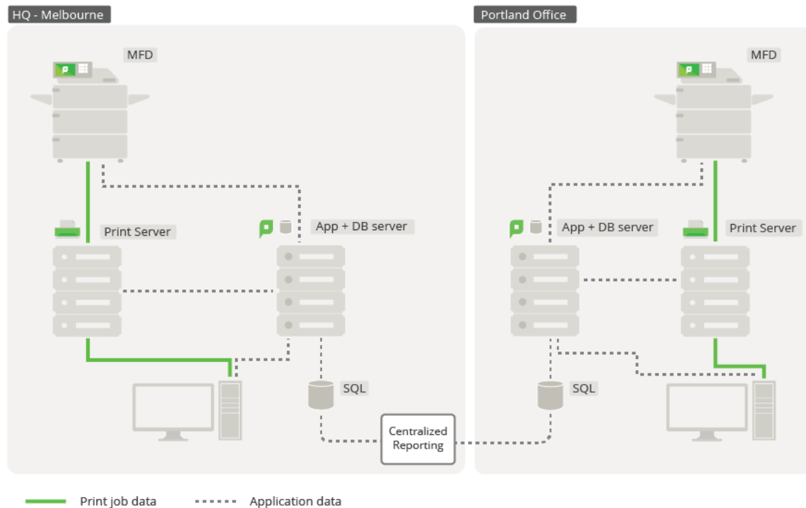
Figure 7: Multi Site/Multi Server deployment
