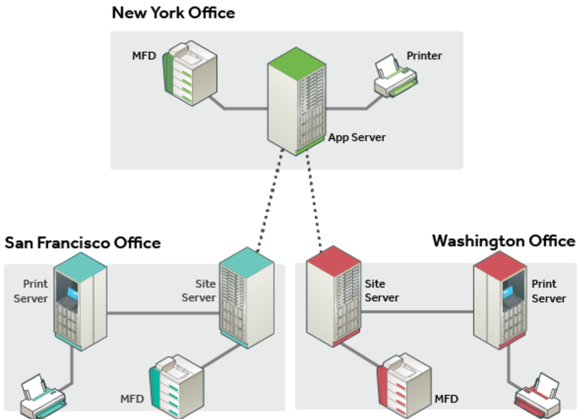
Figure 8: Site Server example
