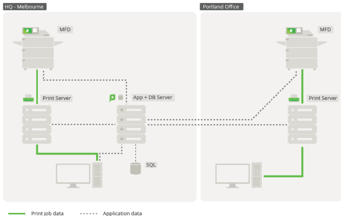
Figure 6: Multiple site / multiple print server deployment
